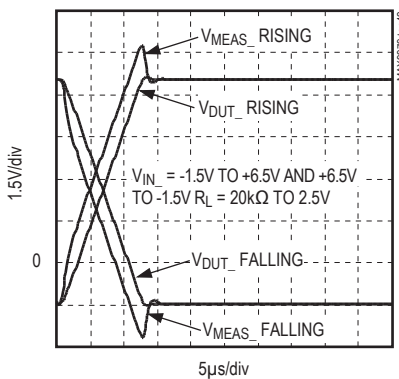
TRANSIENT RESPONSE FVMI RANGE C
