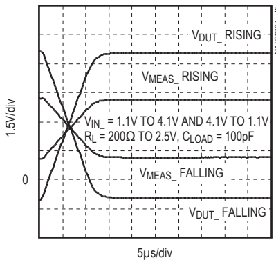
TRANSIENT RESPONSE FIMI RANGE A
